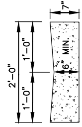
VALLEY GUTTER
