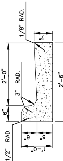
2'-6" CURB AND GUTTER
